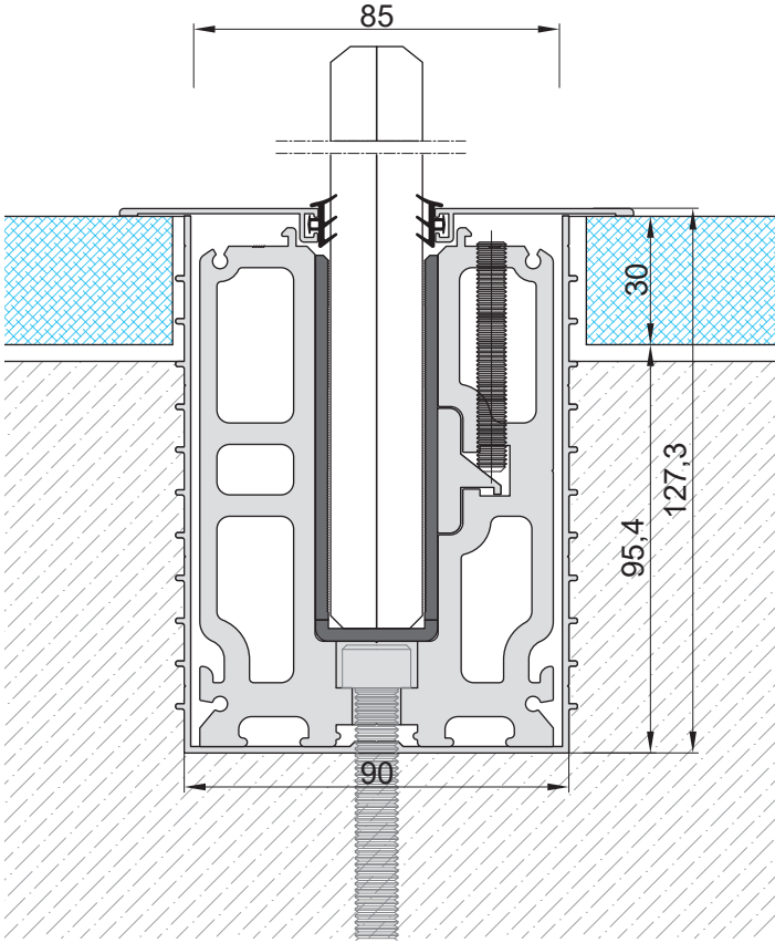
SMART BASE 85-125B GÖMÜLÜ SİSTEM DETAYI 1 10 mm + PVB + 10 mm
